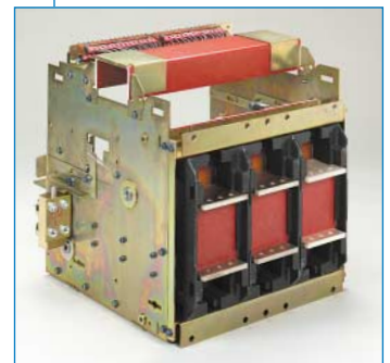
Rear view of integrally-designed cassette showing generous spacing for customer bus connections.
