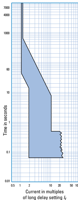
Digitrip 520i/520Mi Long and short delay curves
